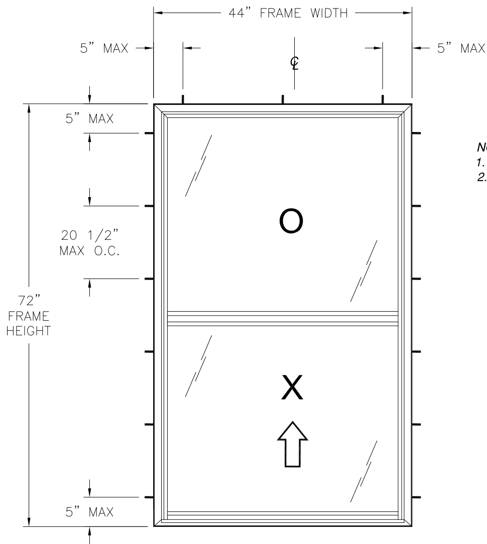
220 VINYL SINGLE HUNG WINDOW EXTERIOR VIEW
