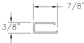
SASH STILES REINFORCEMENT (731-A) ALUMINUM 6005-T5
