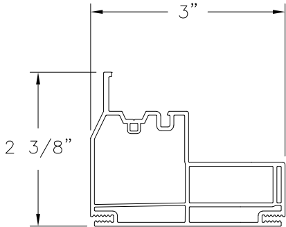
HEAD (9203) EXTRUDED RIGID PVC
