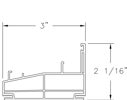
SILL (9202A) EXTRUDED RIGID PVC
